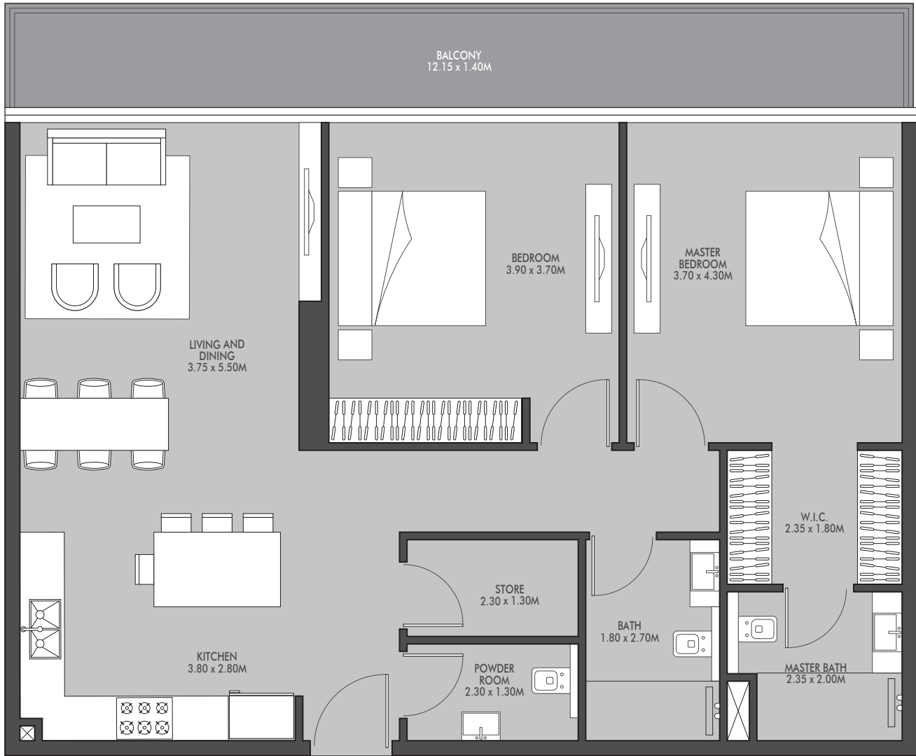
UNIT 04 2-BEDROOM TYPE B
