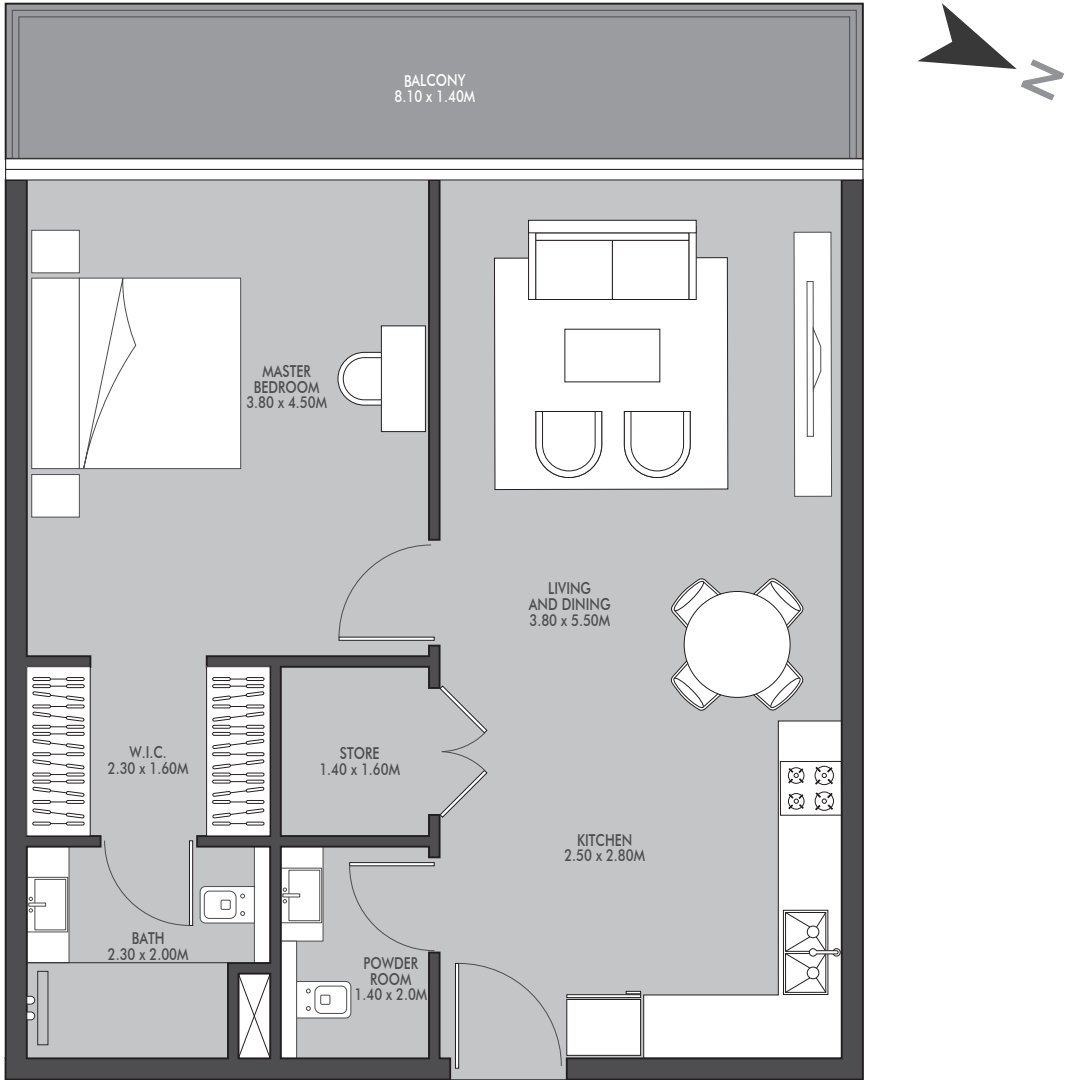
UNIT 07 1-BEDROOM TYPE A
