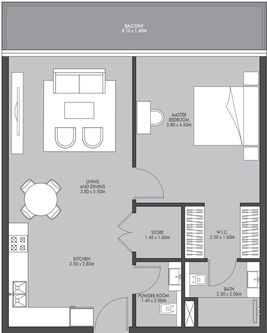
UNIT 10 1-BEDROOM TYPE A
