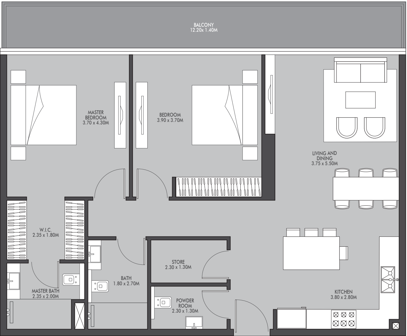
UNIT 03 2-BEDROOM TYPE B
