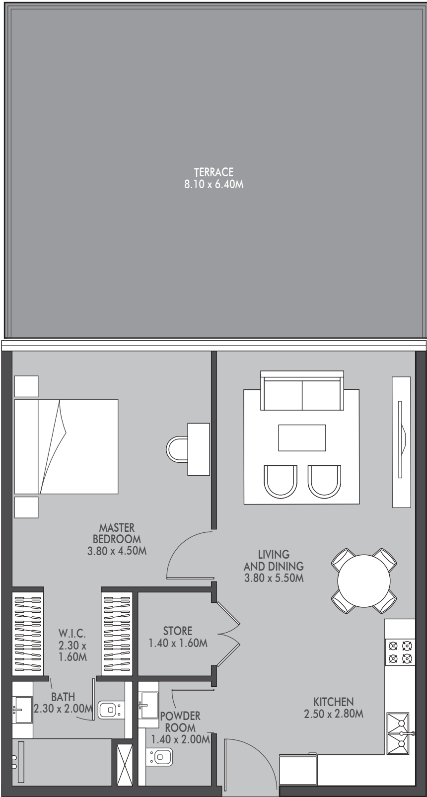
UNIT 12 1-BEDROOM TYPE A
