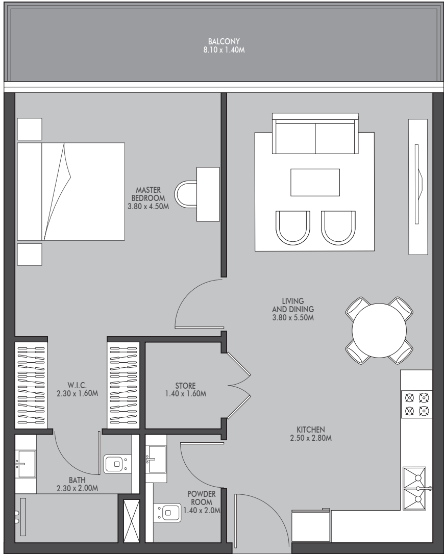
UNIT 12 1-BEDROOM TYPE A
