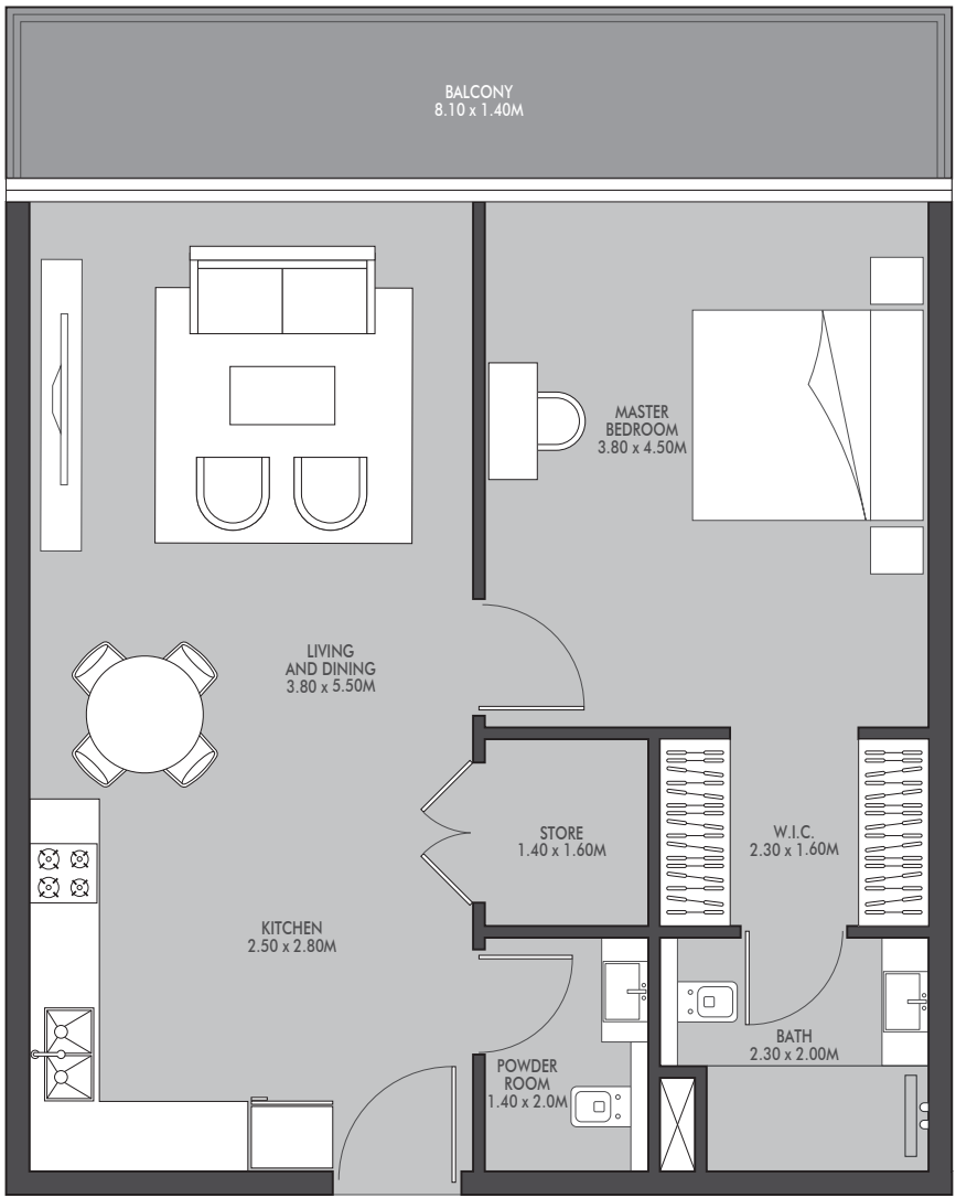
UNIT 05 1-BEDROOM TYPE A
